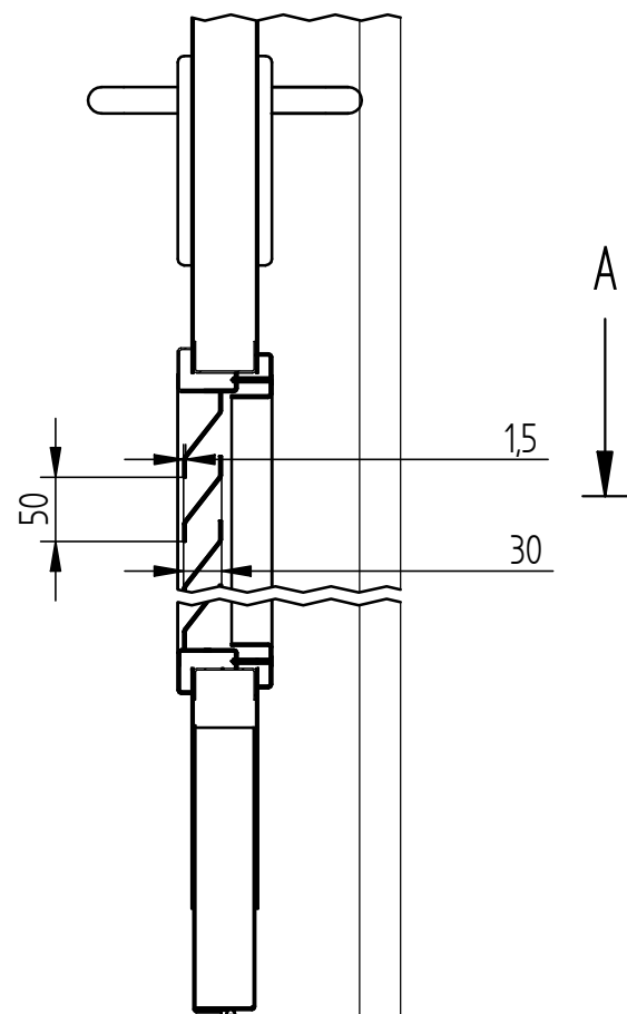
SECTION B-B
