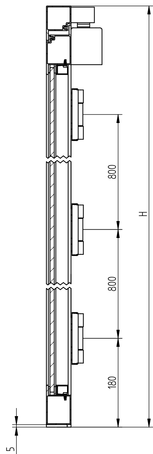
SECTION B-B
